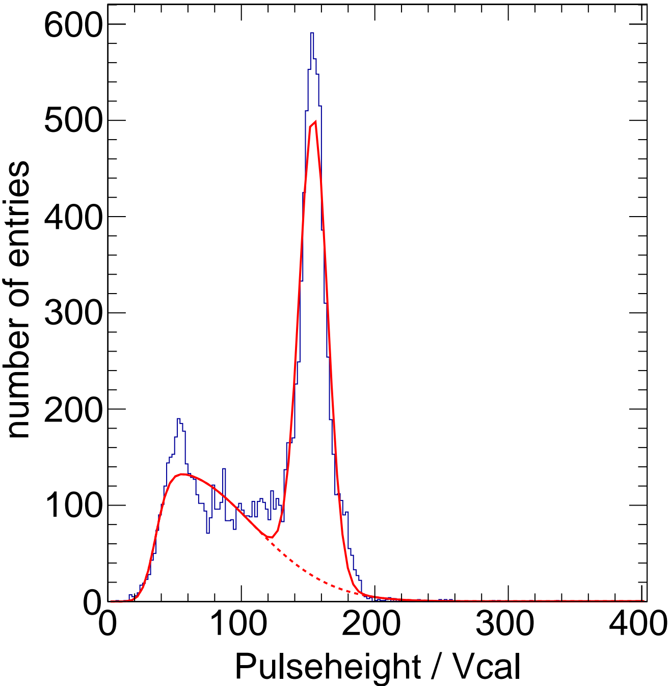
X-ray Calibration - Target Sn Method Spectrum Chip C1
