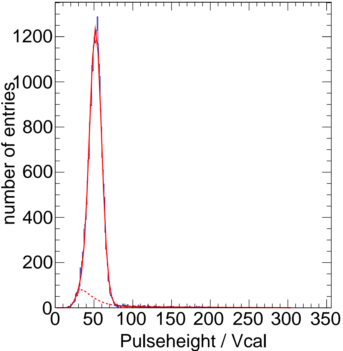
X-ray Calibration - Target Zn Method Spectrum Chip C9
