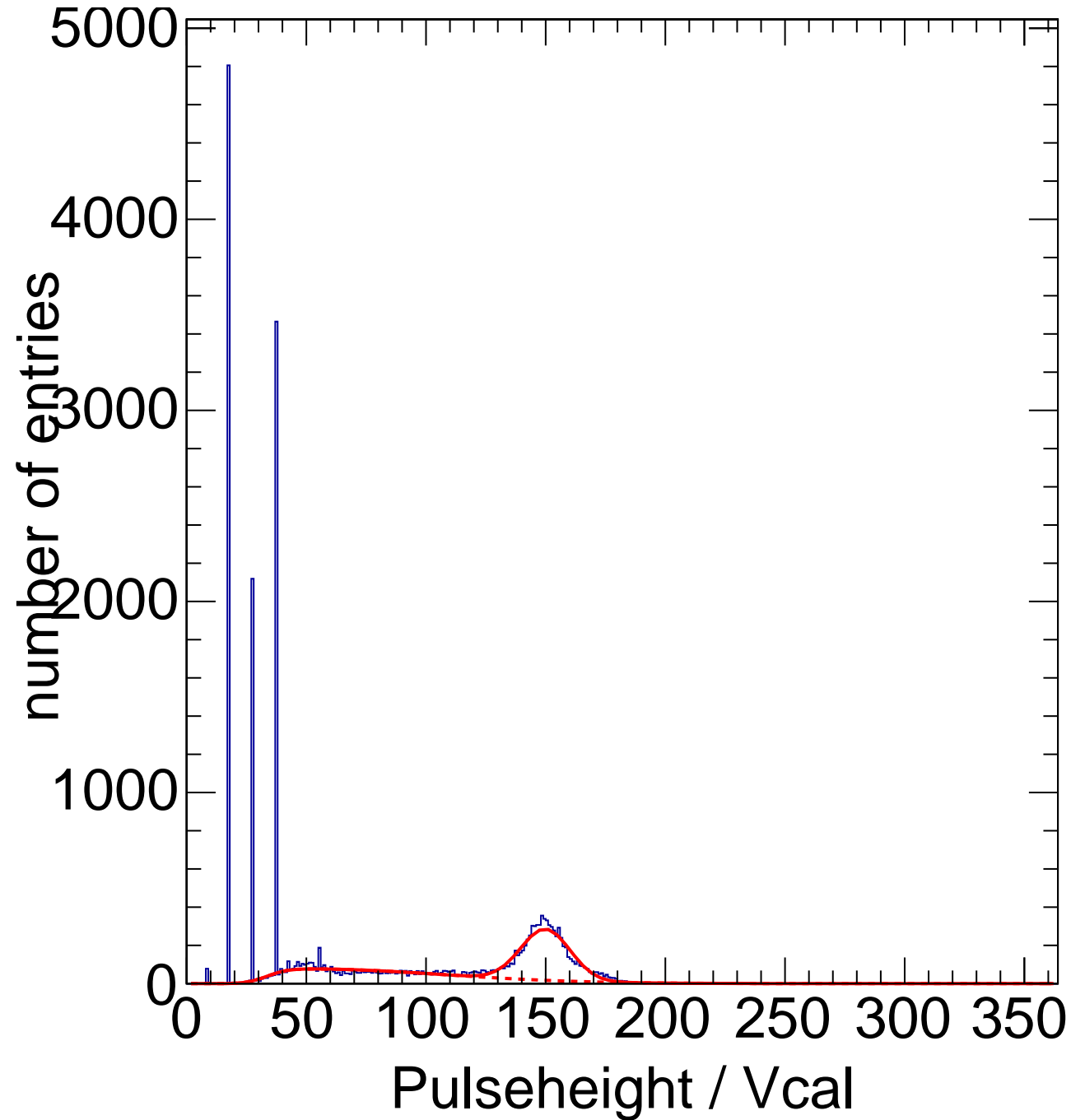
X-ray Calibration - Target Sn Method Spectrum Chip C12
