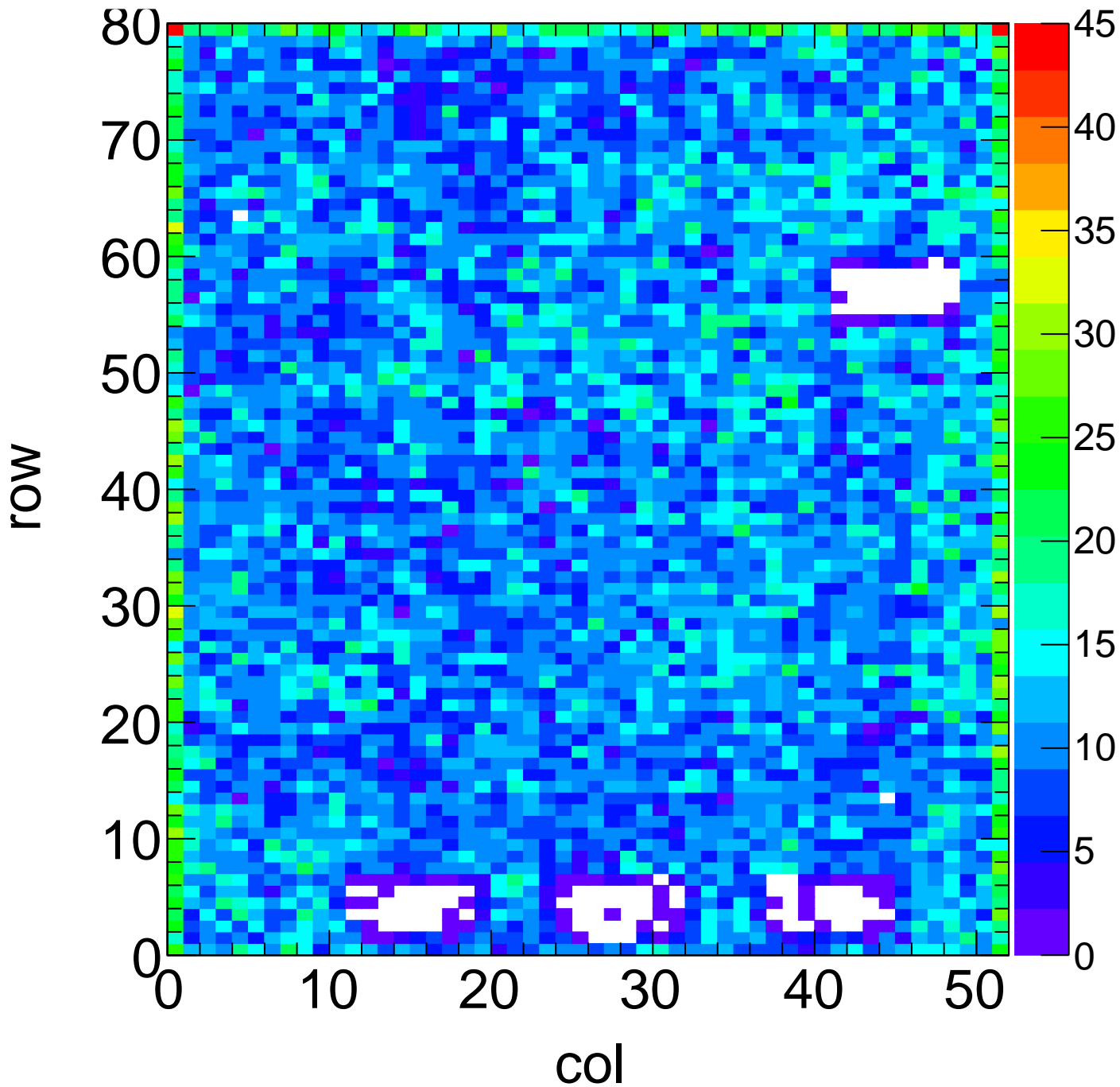
X-ray Hit Map - Target Mo Method Spectrum Chip C4
