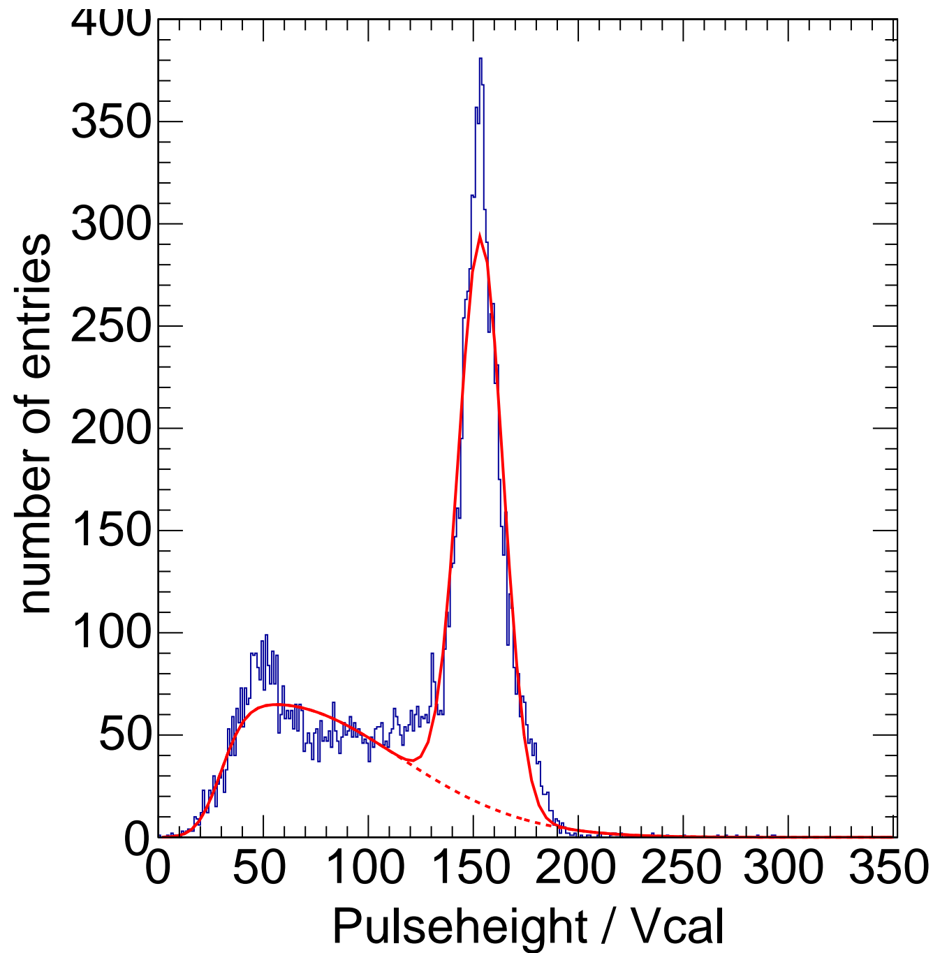
X-ray Calibration - Target Sn Method Spectrum Chip C3
