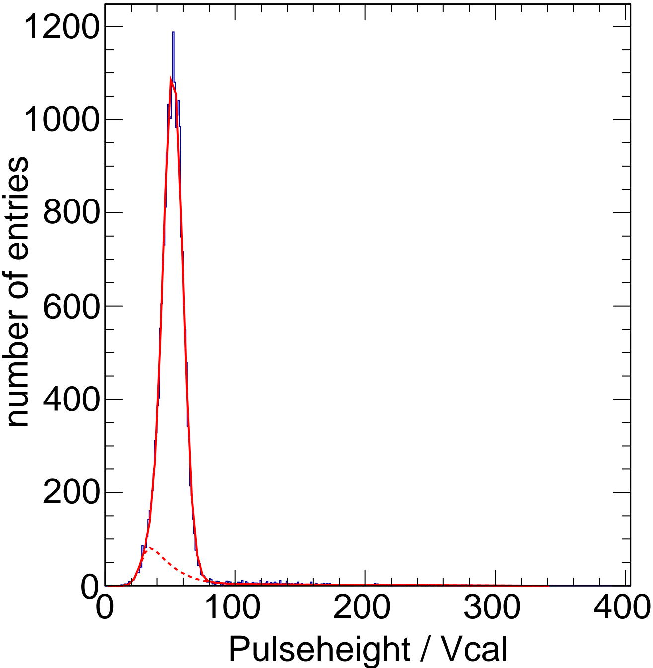
X-ray Calibration - Target Zn Method Spectrum Chip C1
