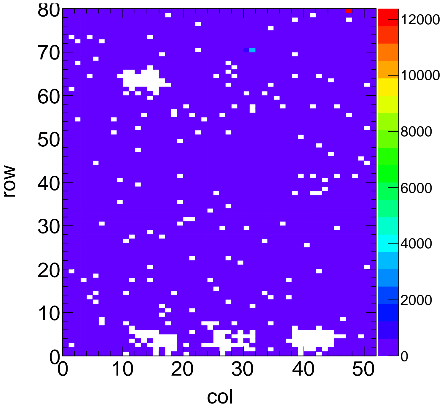
X-ray Hit Map - Target Sn Method Spectrum Chip C3
