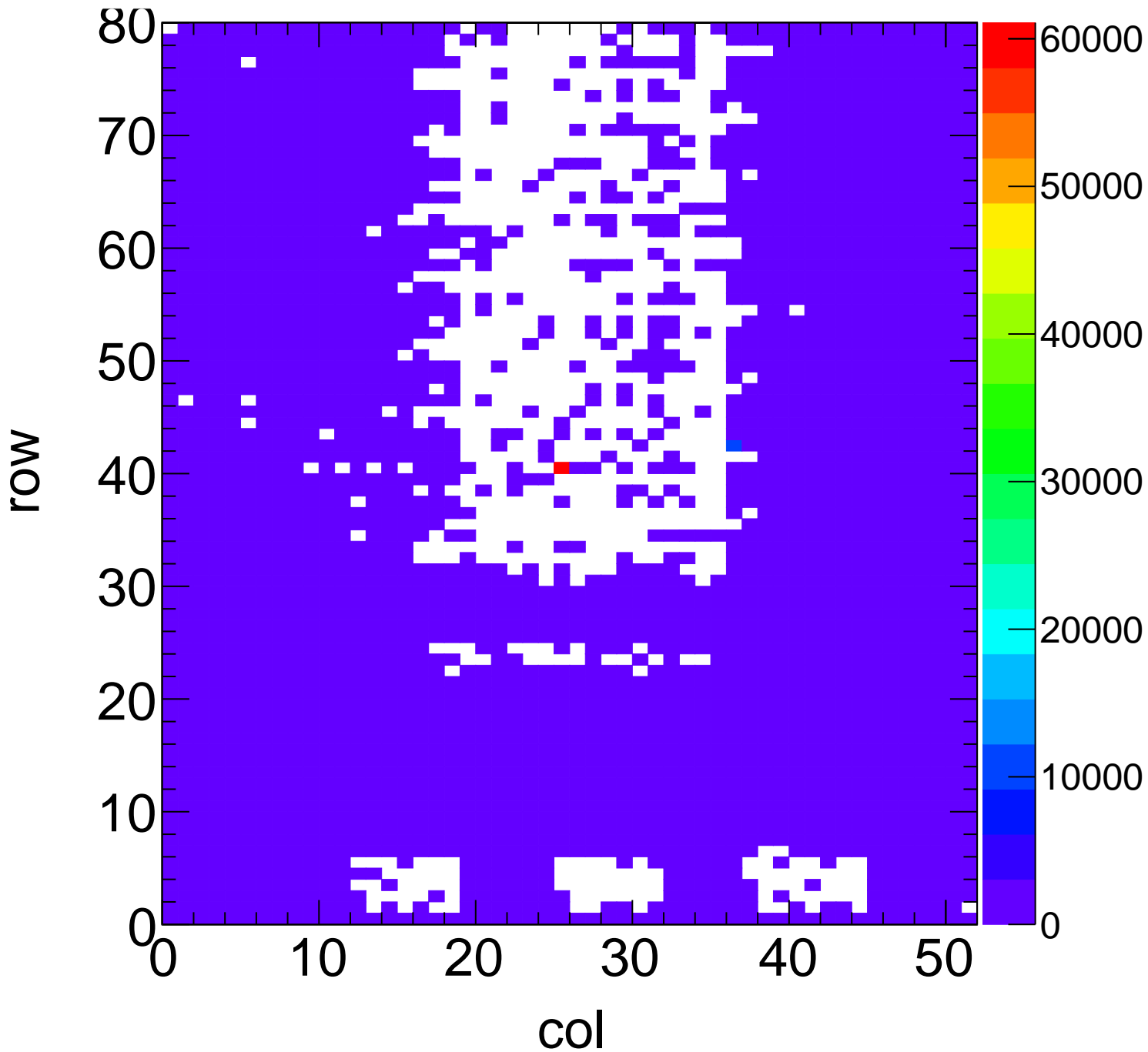
X-ray Hit Map - Target Mo Method Spectrum Chip C2
