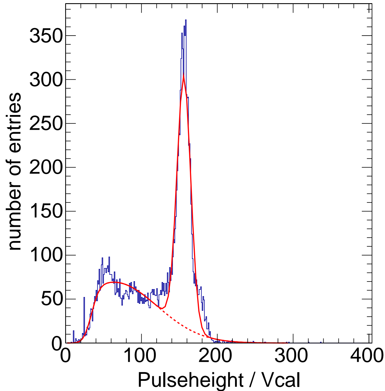
X-ray Calibration - Target Sn Method Spectrum Chip C11
