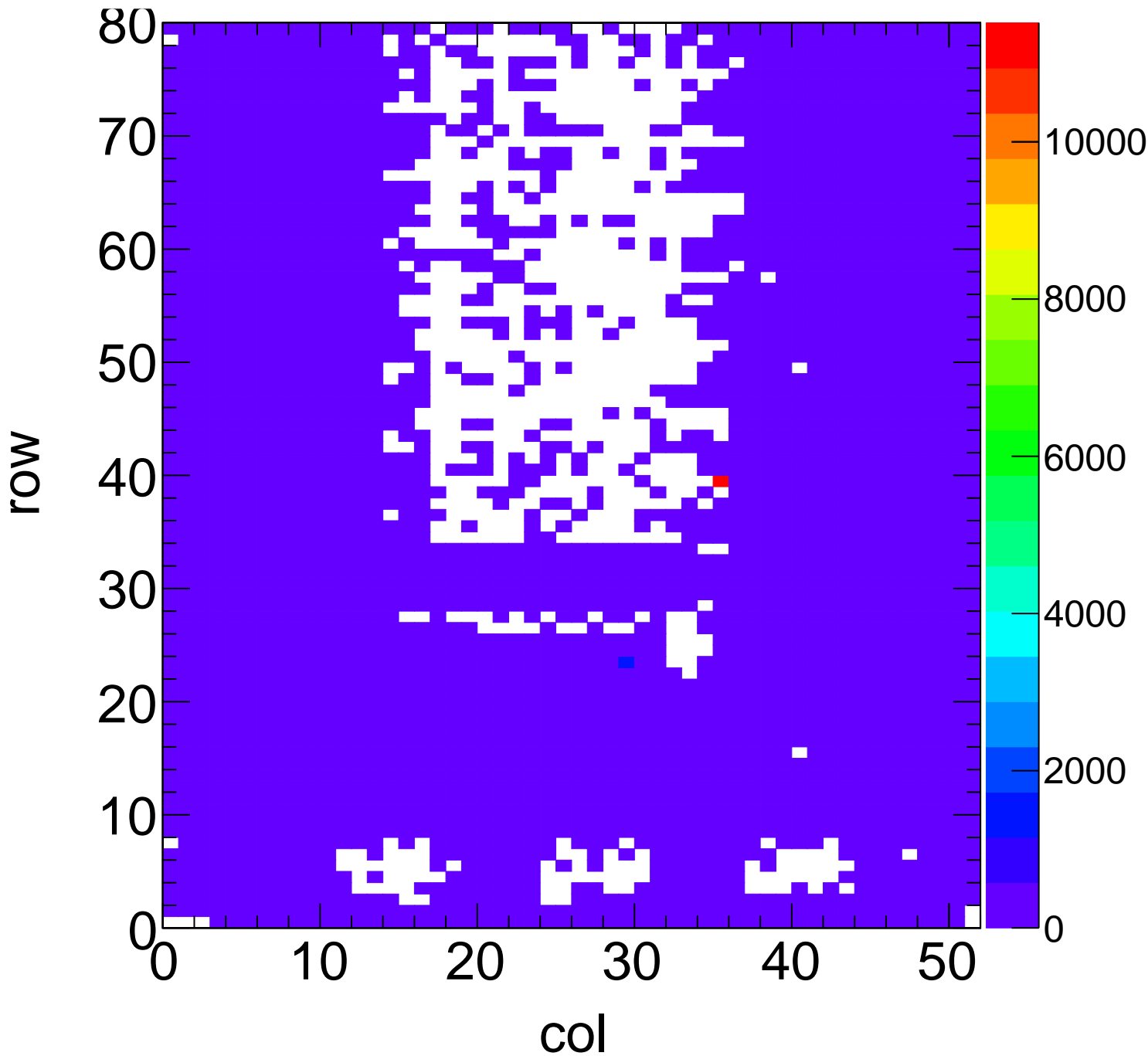
X-ray Hit Map - Target Mo Method Spectrum Chip C13
