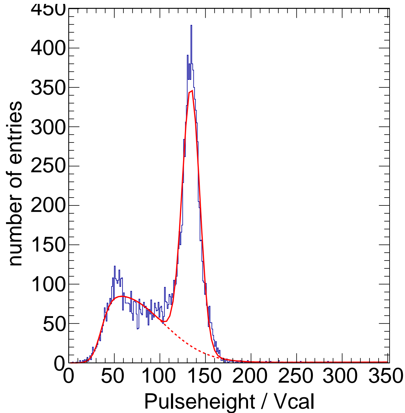
X-ray Calibration - Target Ag Method Spectrum Chip C2
