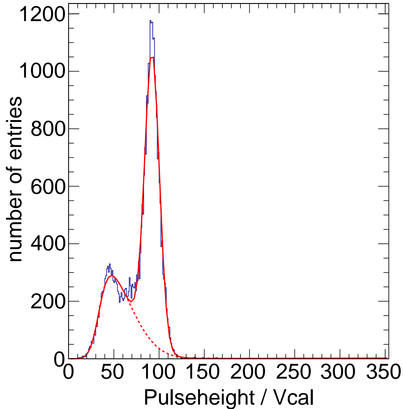
X-ray Calibration - Target Mo Method Spectrum Chip C0
