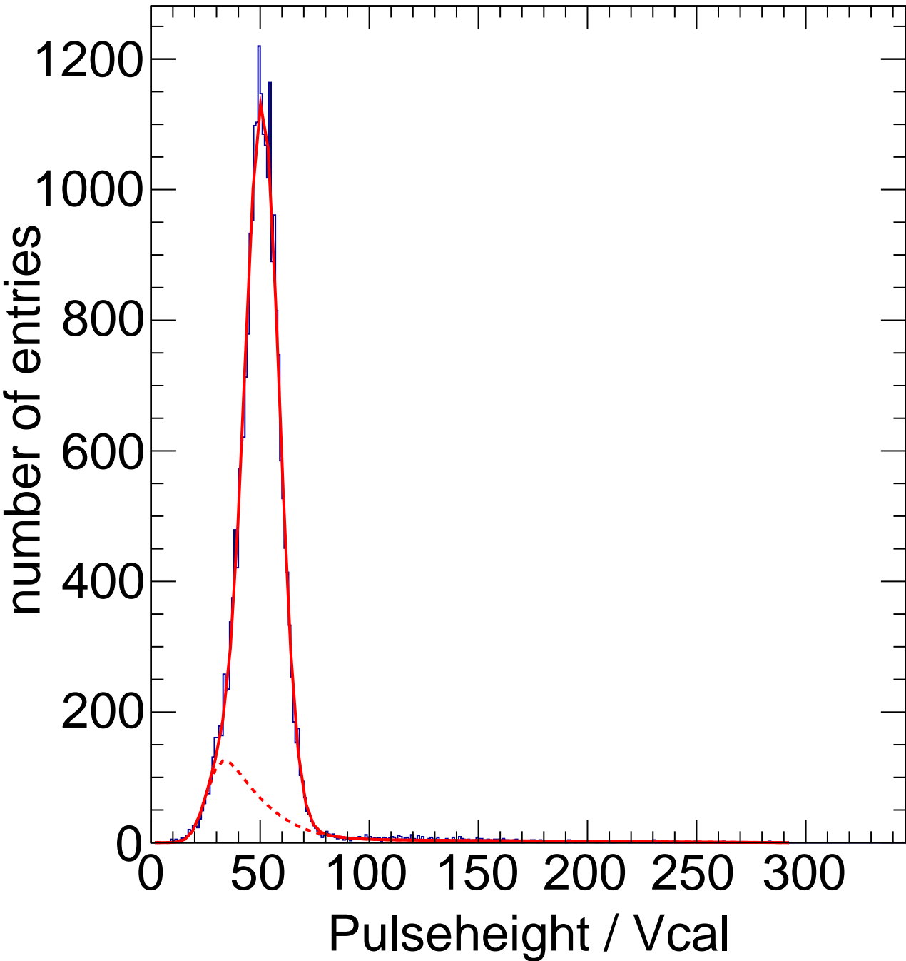
X-ray Calibration - Target Zn Method Spectrum Chip C4
