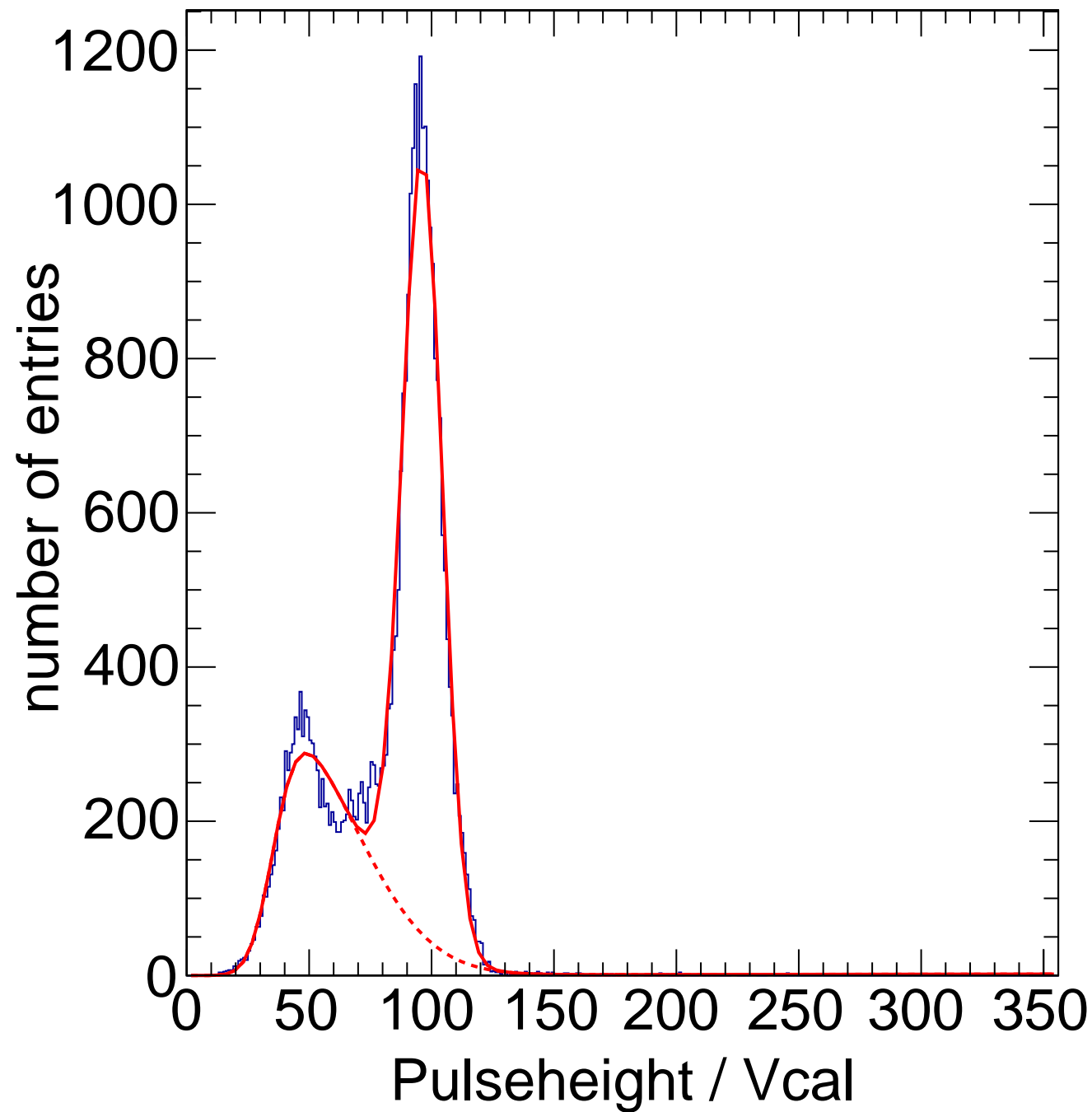
X-ray Calibration - Target Mo Method Spectrum Chip C14
