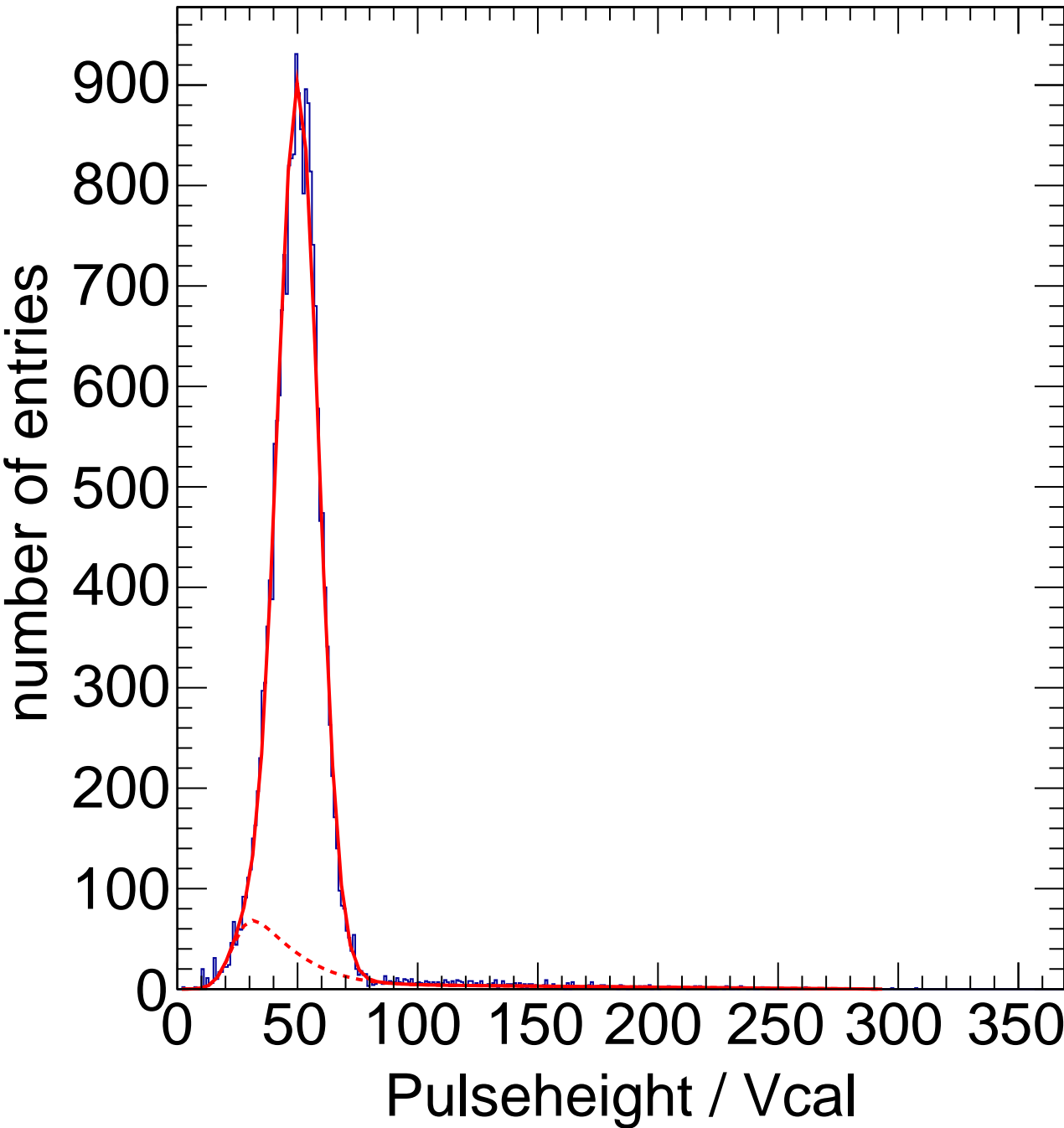
X-ray Calibration - Target Zn Method Spectrum Chip C1
