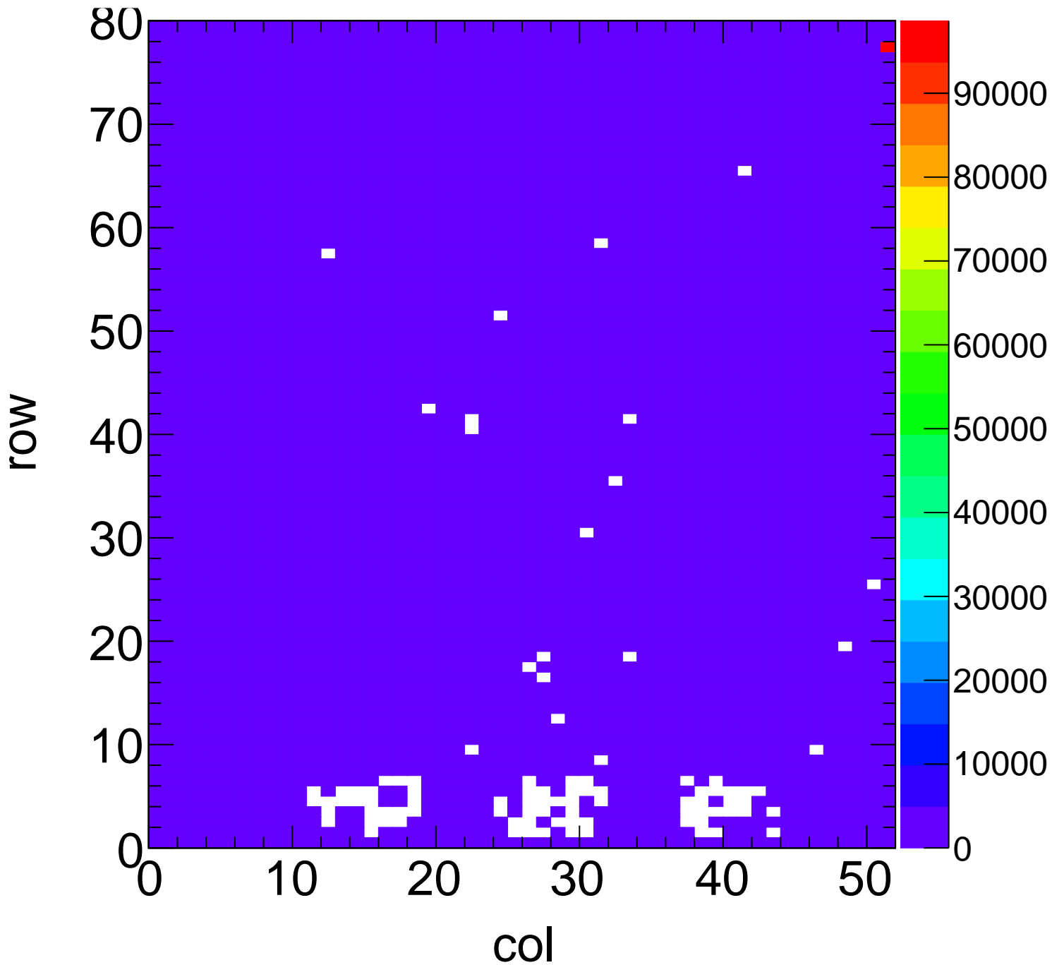
X-ray Hit Map - Target Ag Method Spectrum Chip C5
