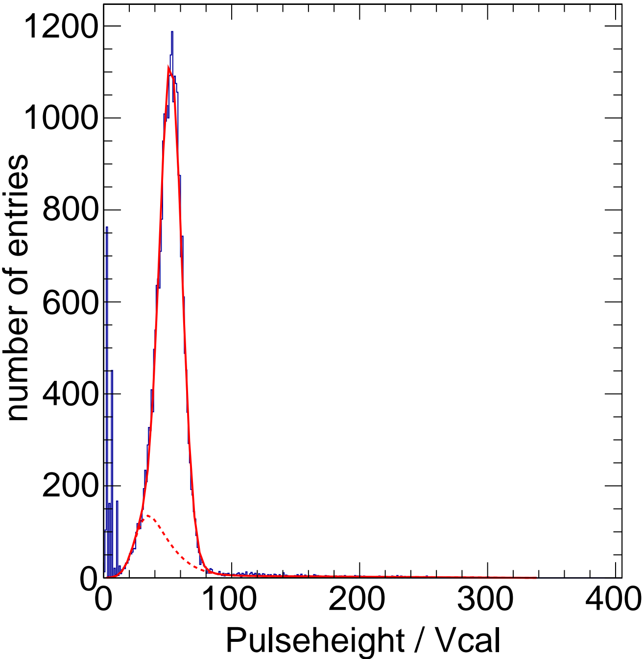
X-ray Calibration - Target Zn Method Spectrum Chip C4
