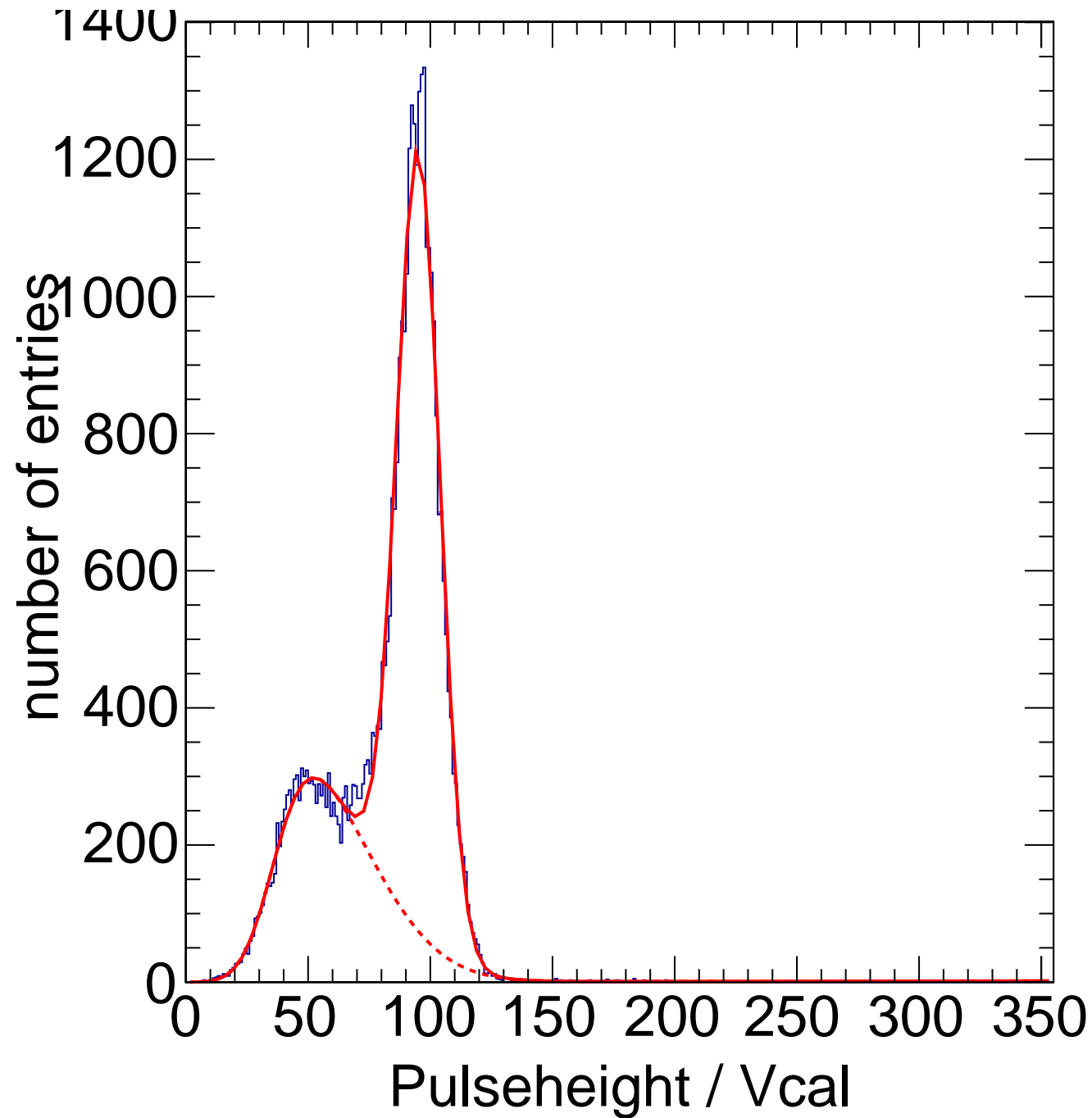
X-ray Calibration - Target Mo Method Spectrum Chip C9
