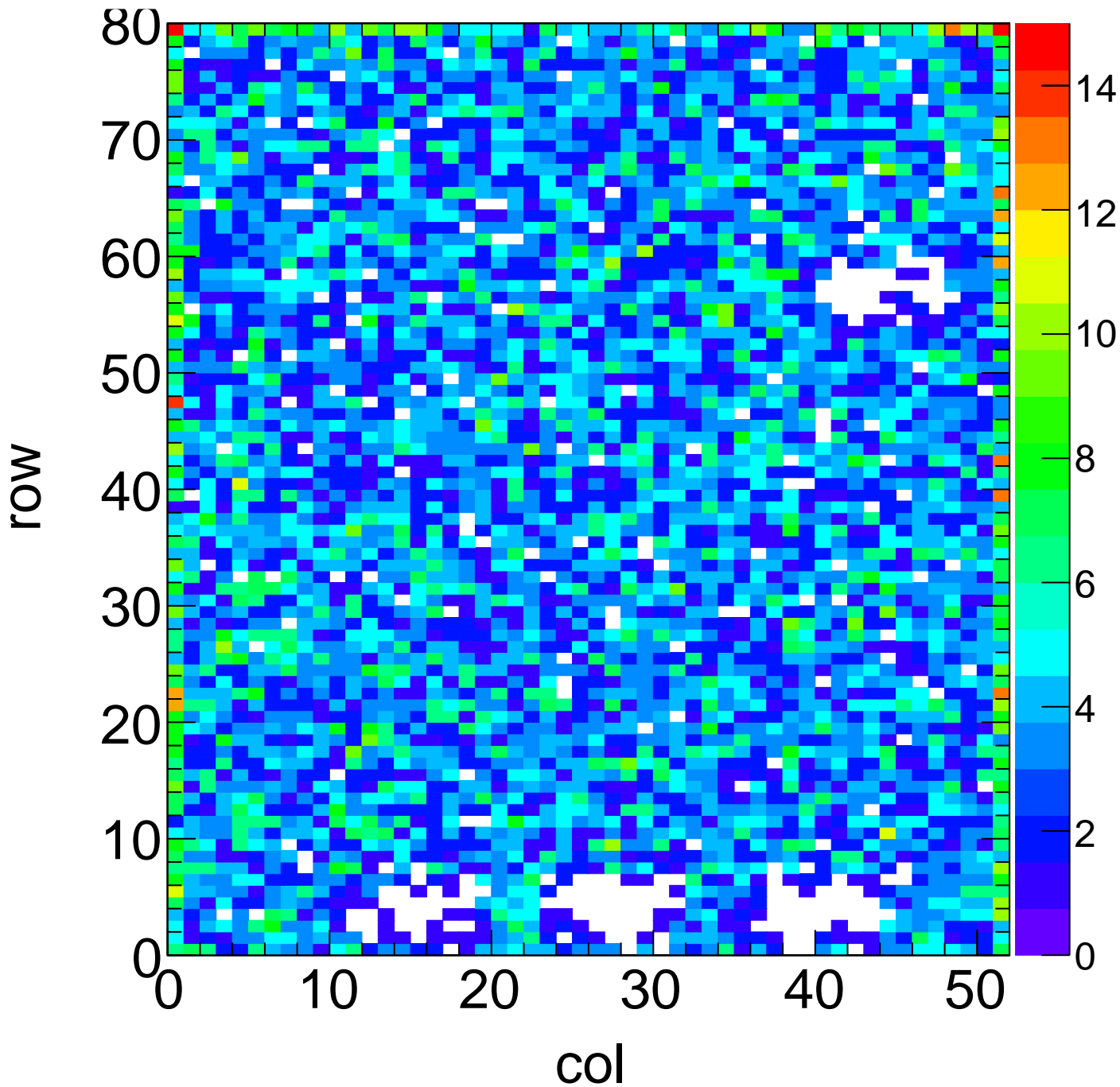
X-ray Hit Map - Target Sn Method Spectrum Chip C4
