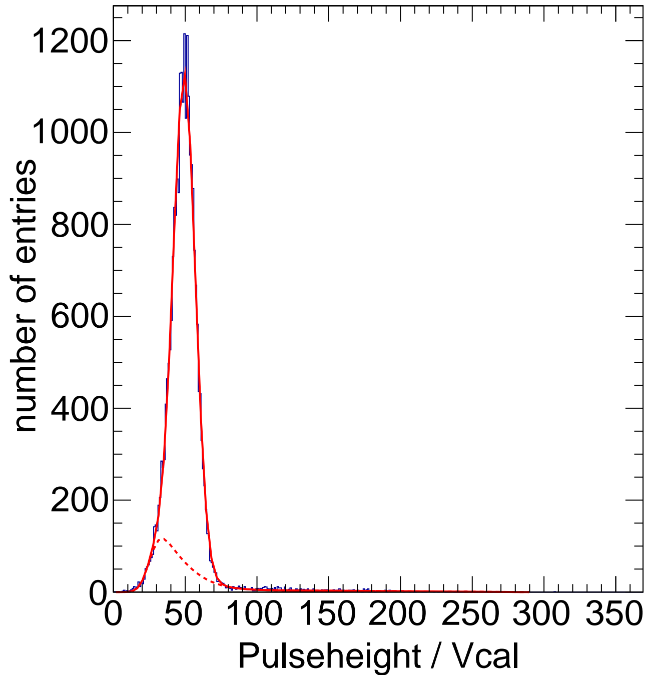
X-ray Calibration - Target Zn Method Spectrum Chip C11
