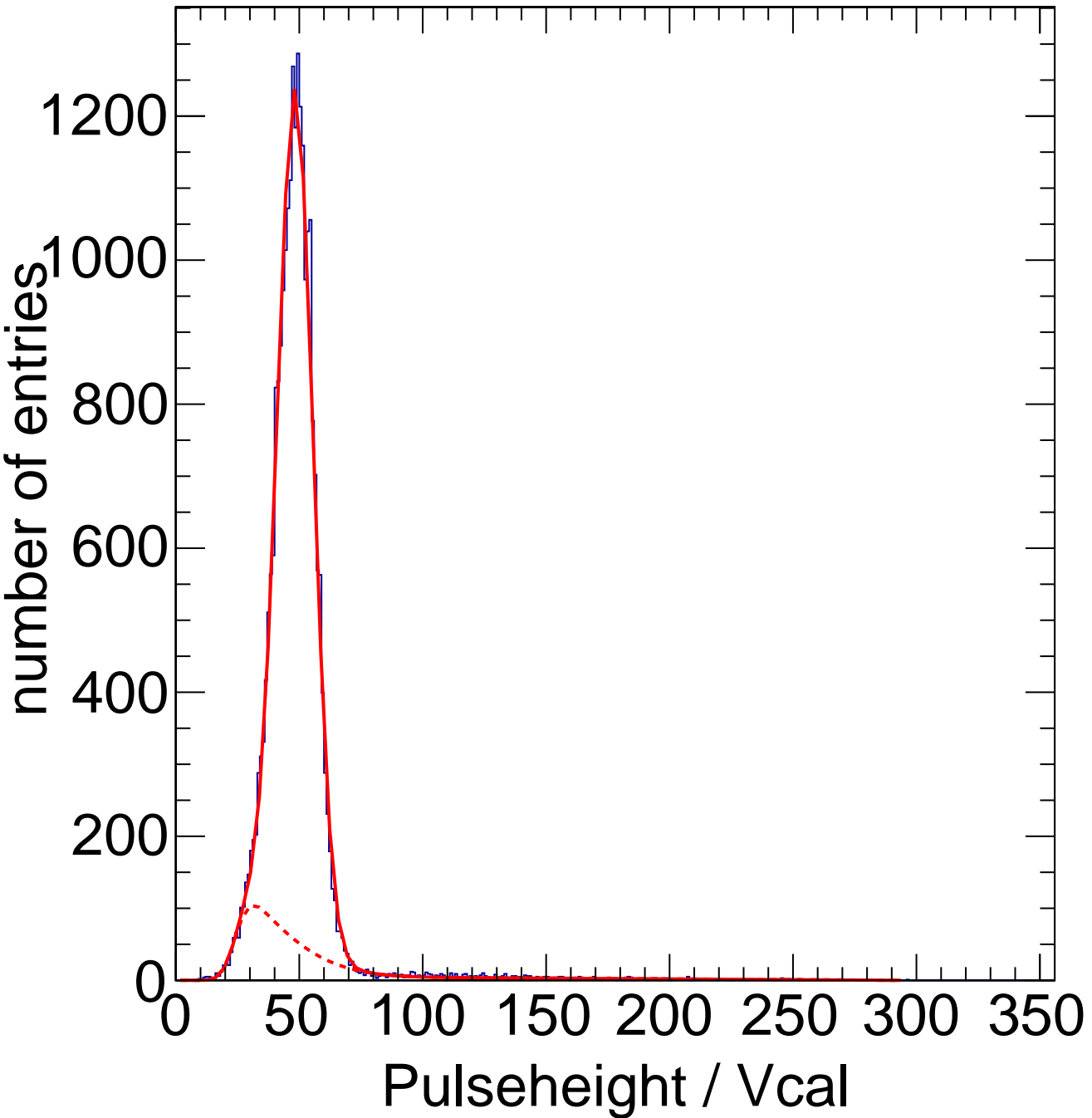
X-ray Calibration - Target Zn Method Spectrum Chip C7
