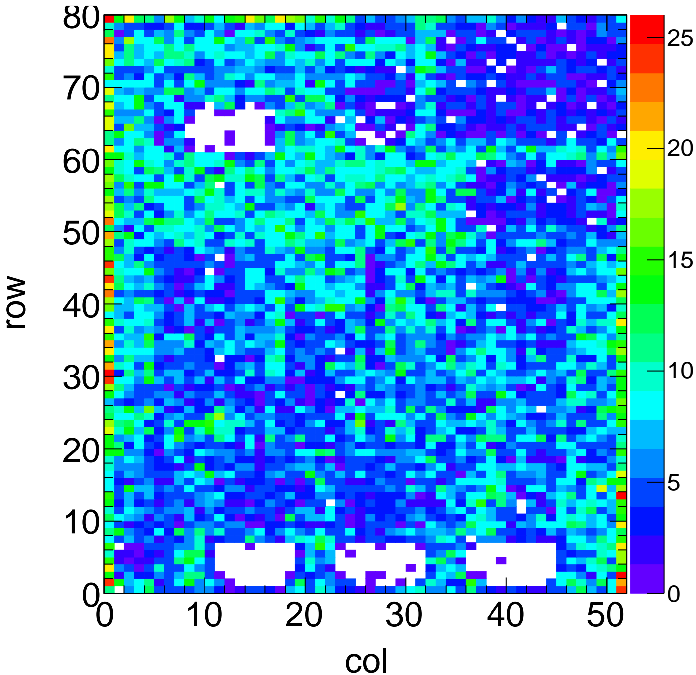
X-ray Hit Map - Target Zn Method Spectrum Chip C3
