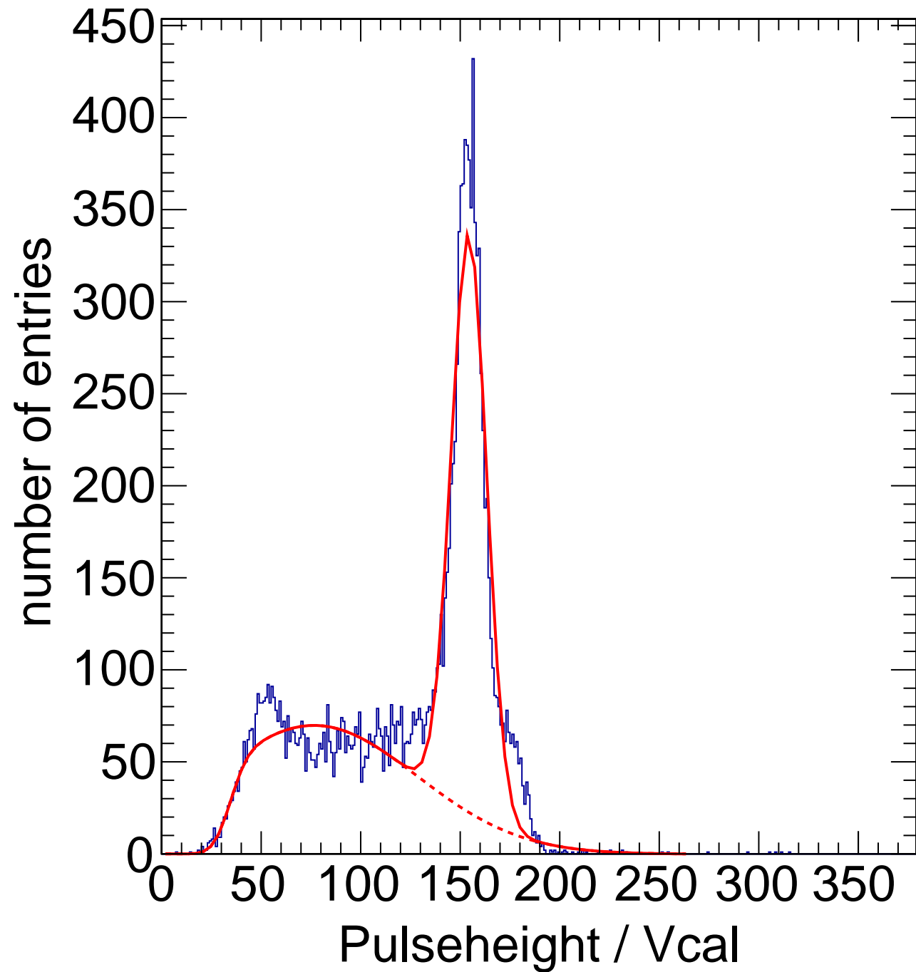
X-ray Calibration - Target Sn Method Spectrum Chip C7
