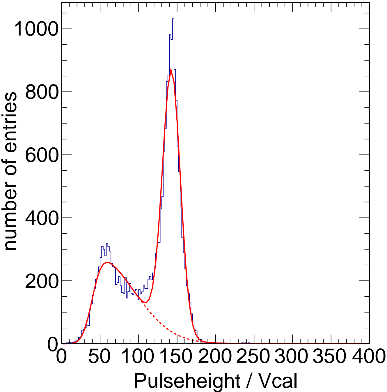
X-ray Calibration - Target Ag Method Spectrum Chip C1
