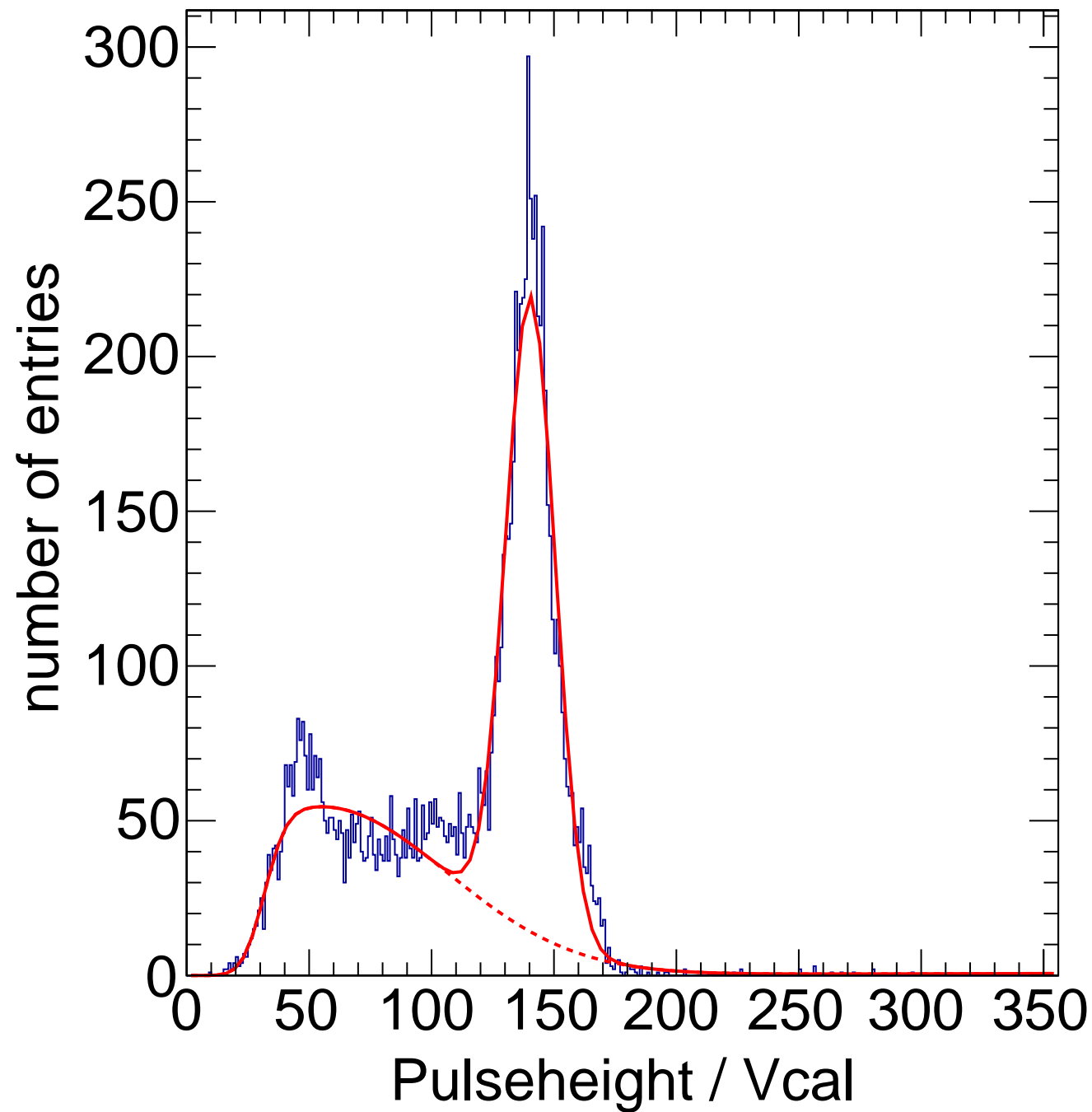
X-ray Calibration - Target Sn Method Spectrum Chip C2
