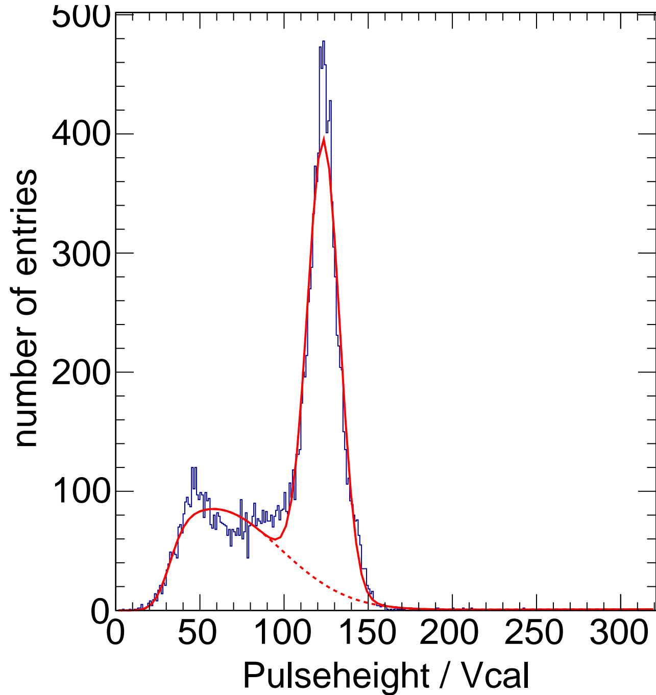
X-ray Calibration - Target Ag Method Spectrum Chip C2
