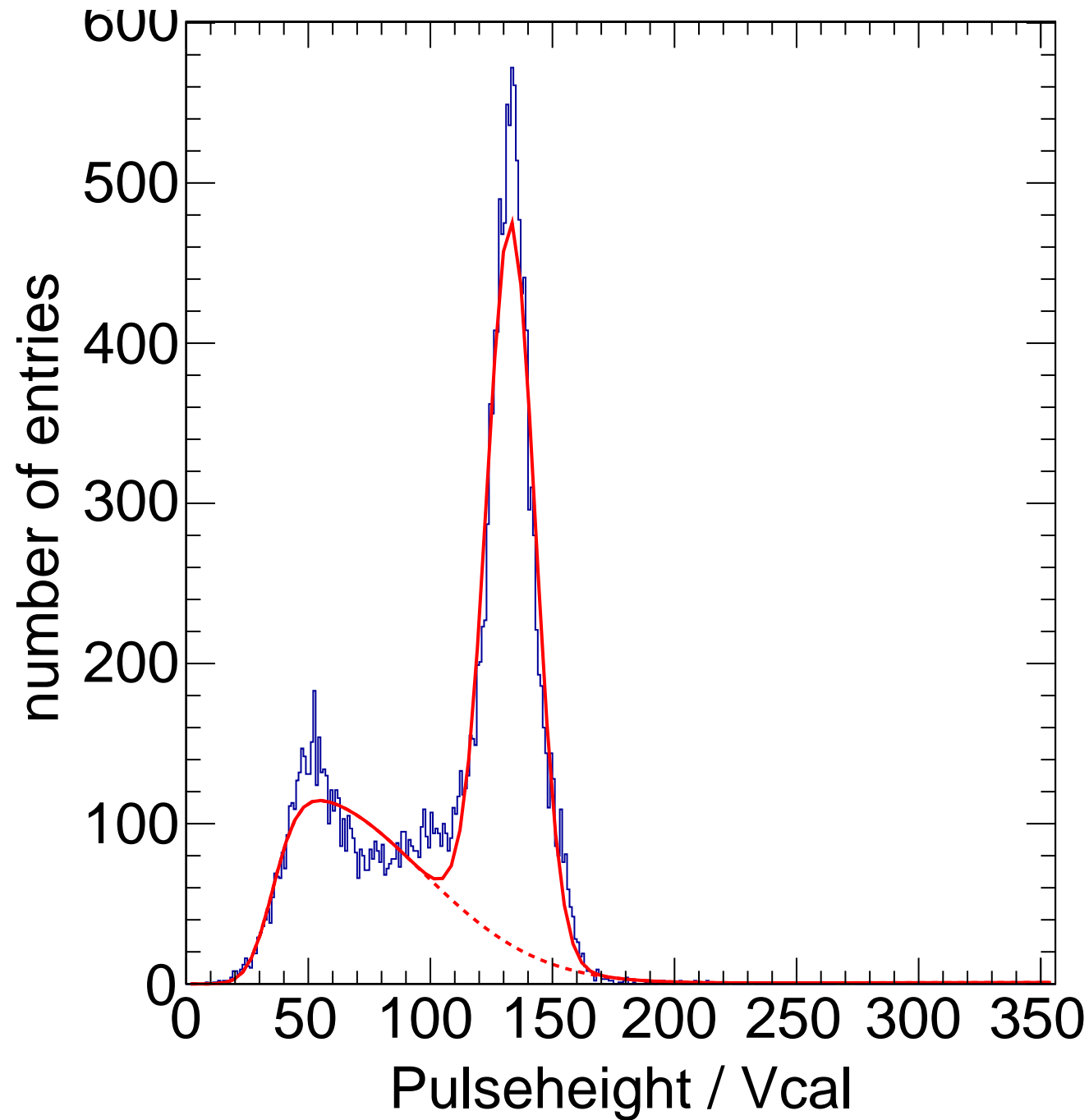
X-ray Calibration - Target Ag Method Spectrum Chip C15
