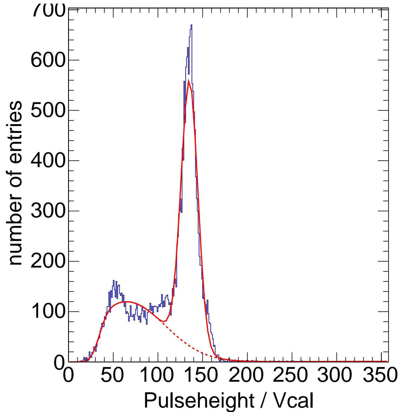
X-ray Calibration - Target Ag Method Spectrum Chip C10
