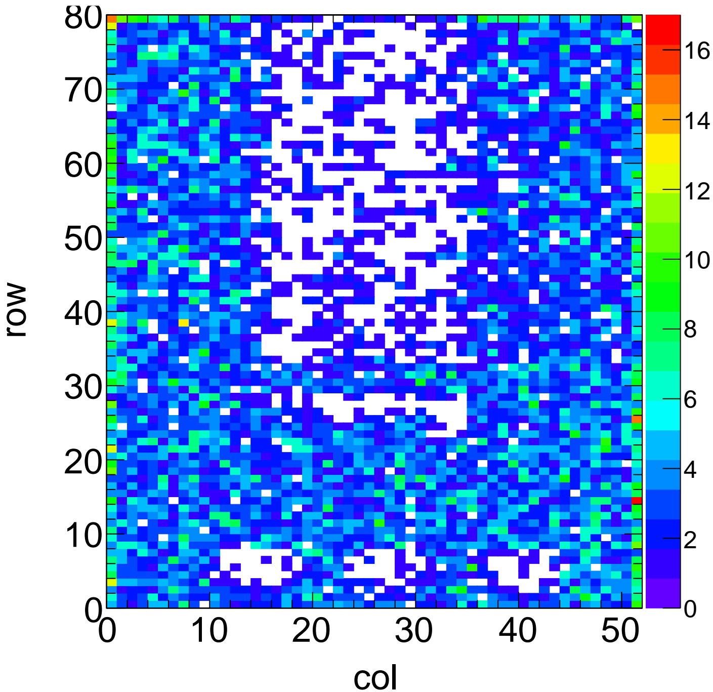
X-ray Hit Map - Target Sn Method Spectrum Chip C13
