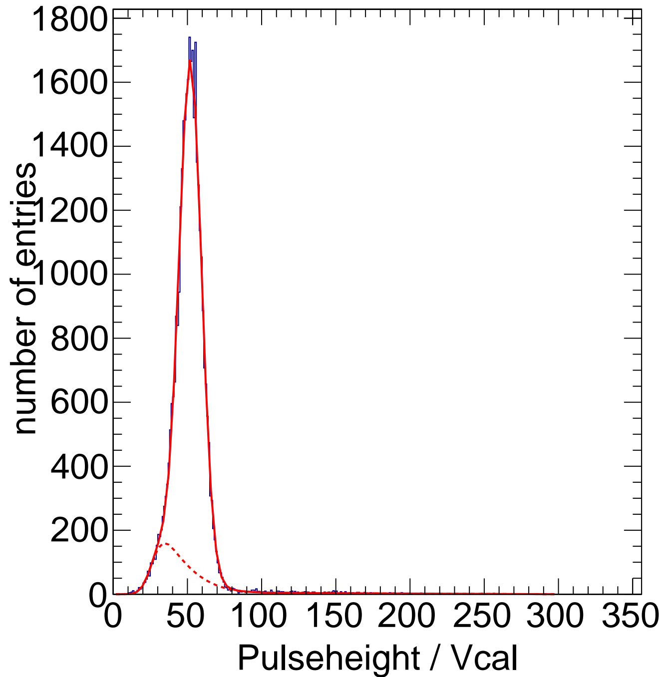
X-ray Calibration - Target Zn Method Spectrum Chip C10
