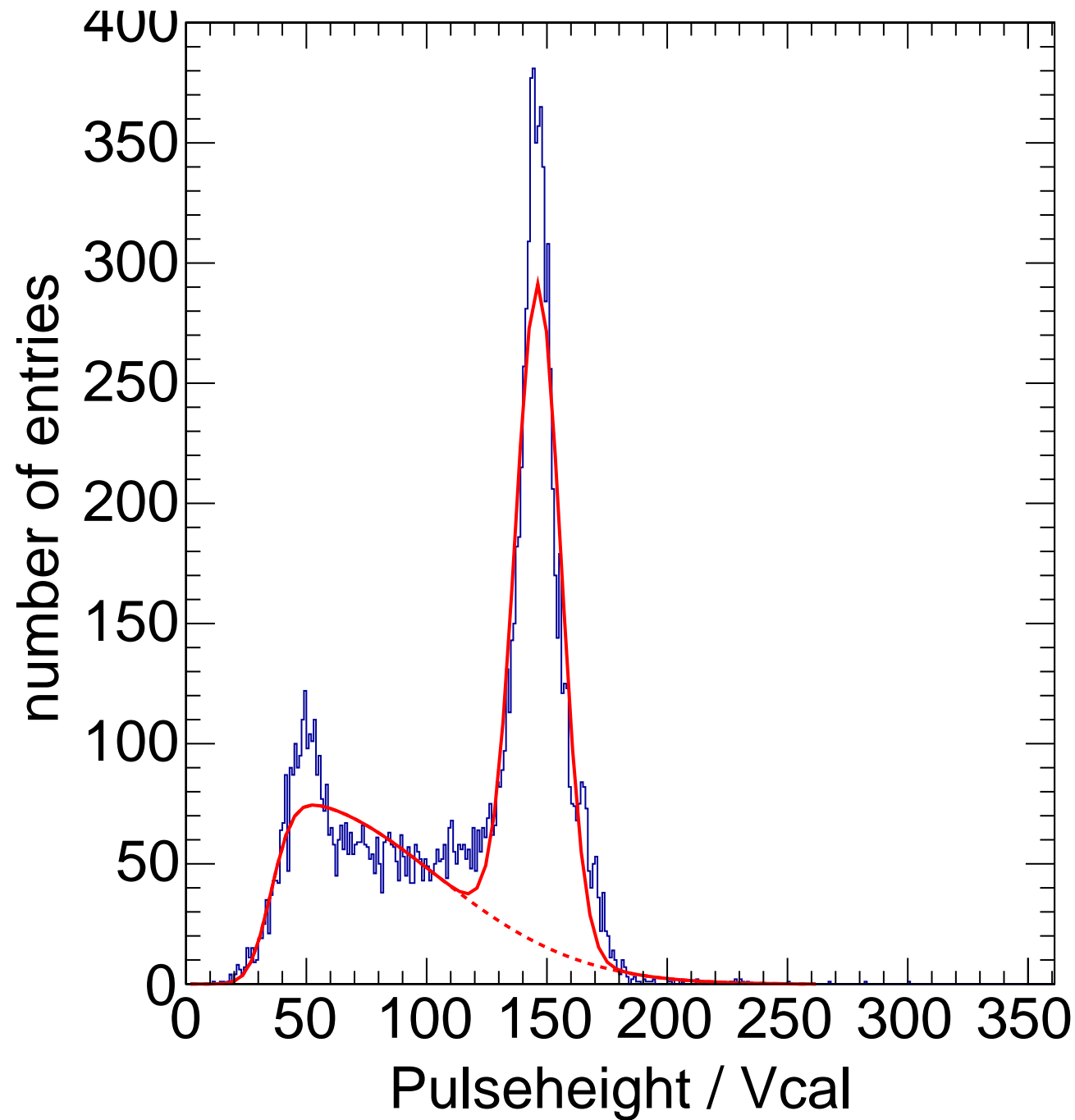
X-ray Calibration - Target Sn Method Spectrum Chip C0
