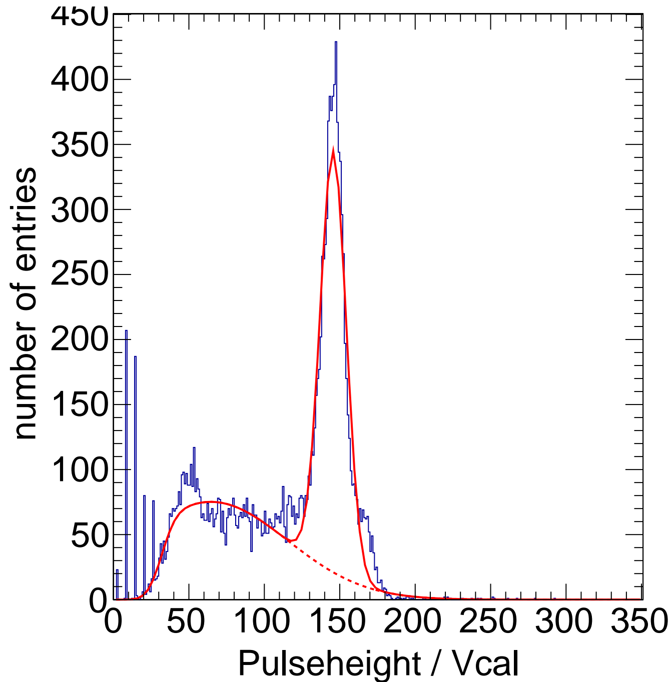
X-ray Calibration - Target Sn Method Spectrum Chip C10
