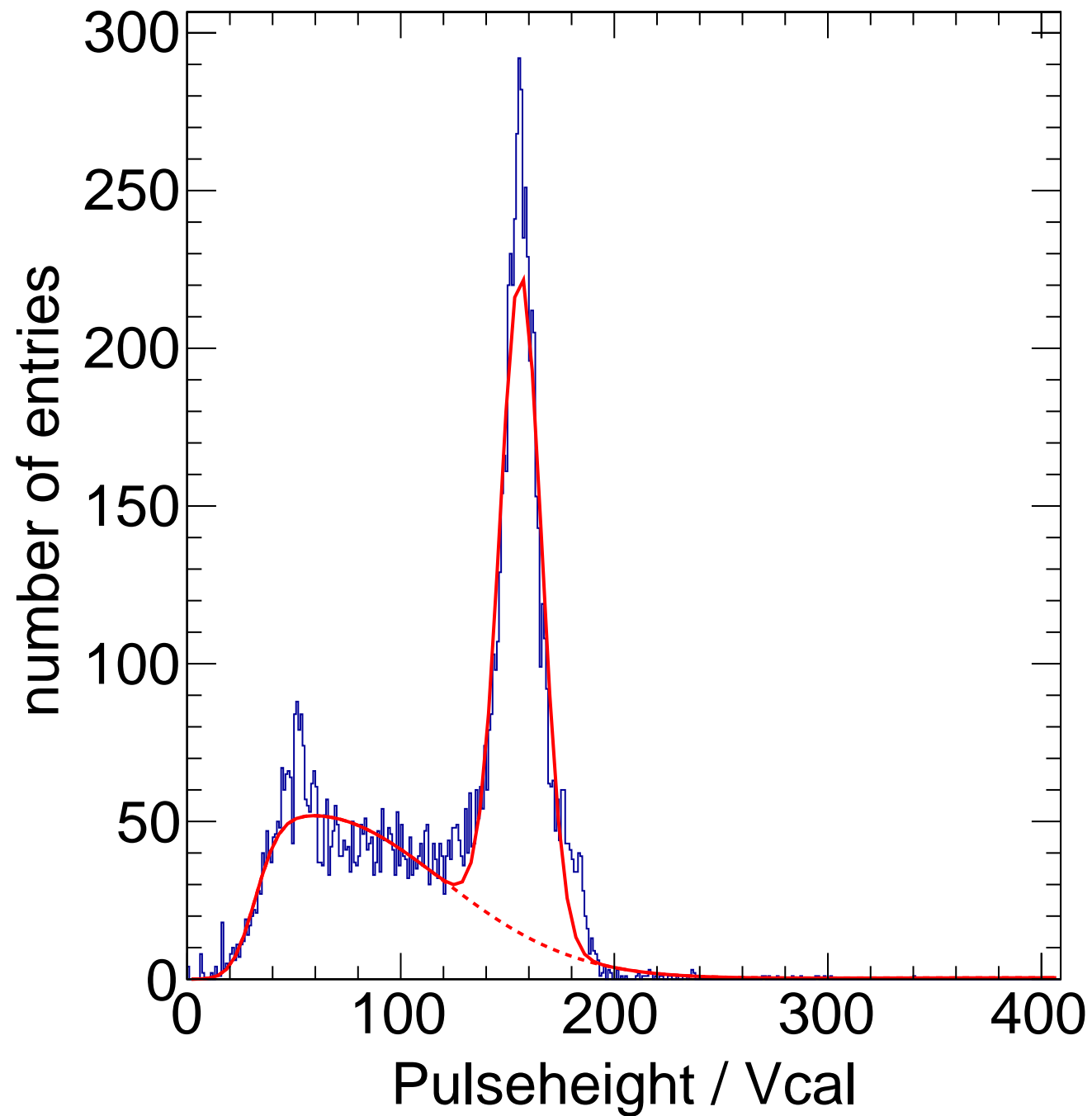
X-ray Calibration - Target Sn Method Spectrum Chip C13
