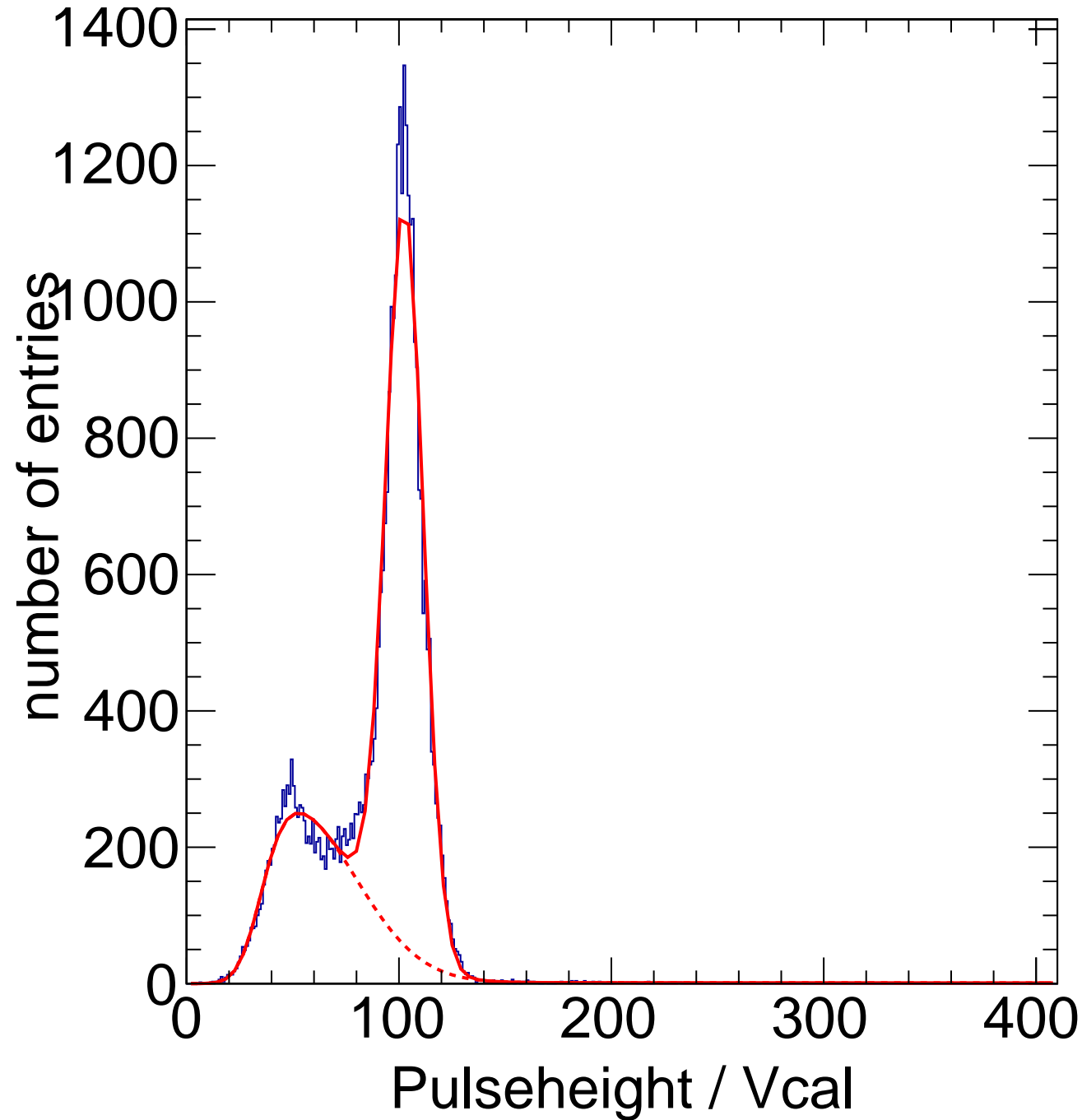
X-ray Calibration - Target Mo Method Spectrum Chip C4
