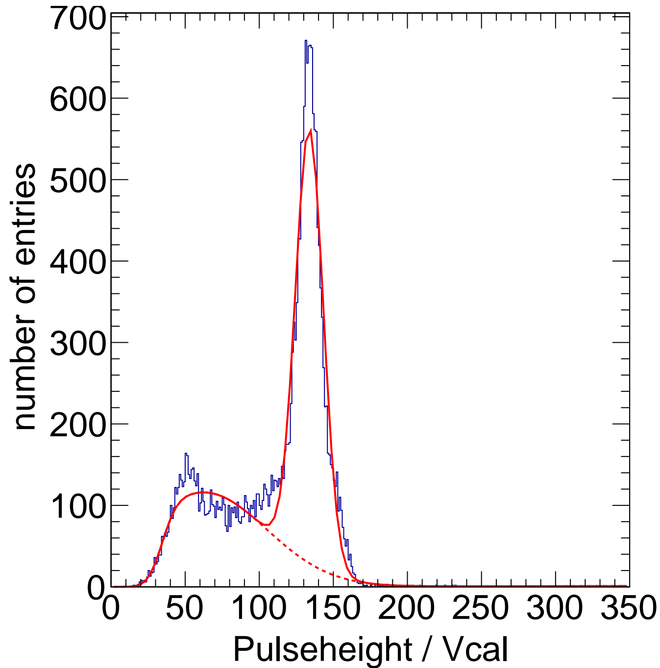
X-ray Calibration - Target Ag Method Spectrum Chip C5
