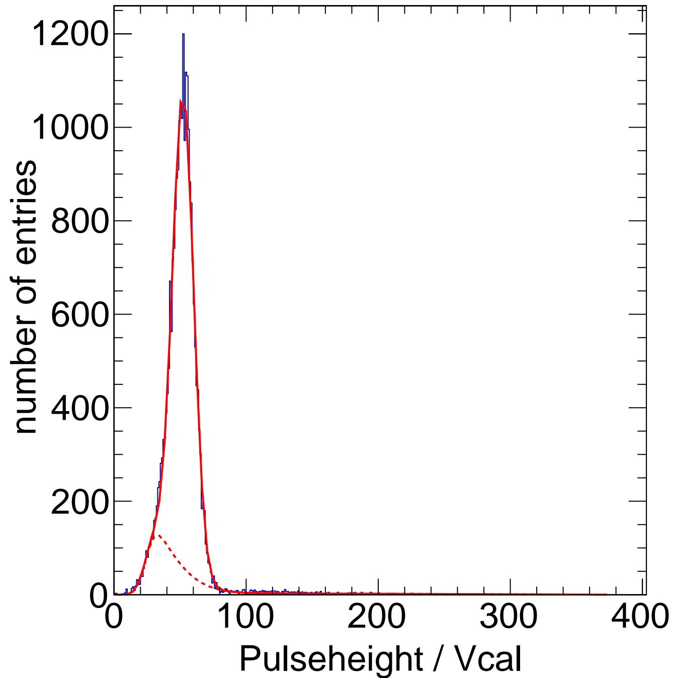
X-ray Calibration - Target Zn Method Spectrum Chip C12
