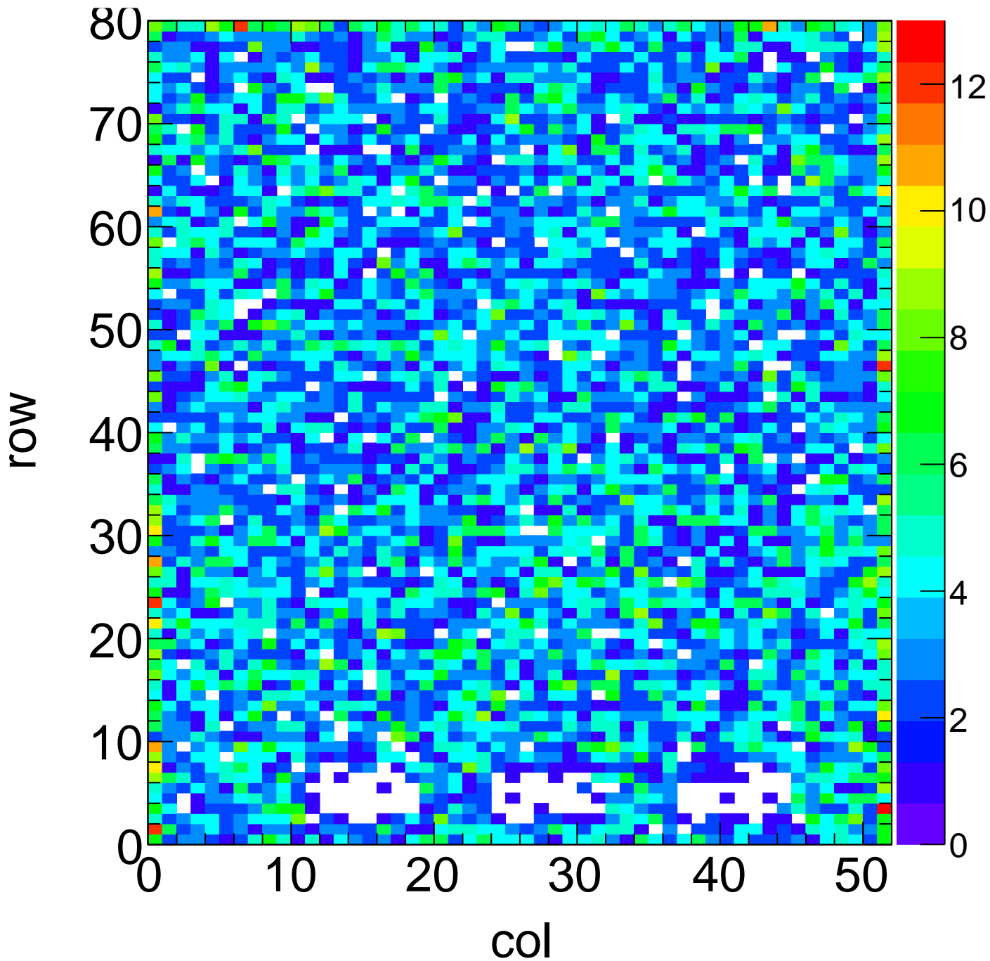
X-ray Hit Map - Target Sn Method Spectrum Chip C14
