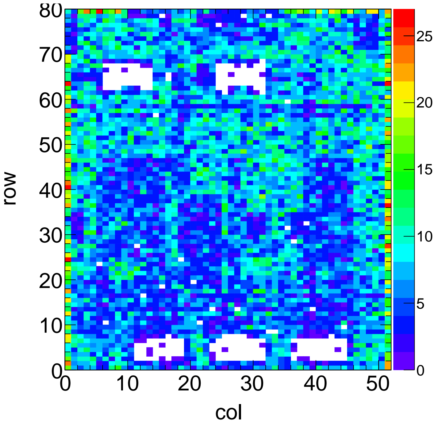
X-ray Hit Map - Target Zn Method Spectrum Chip C9
