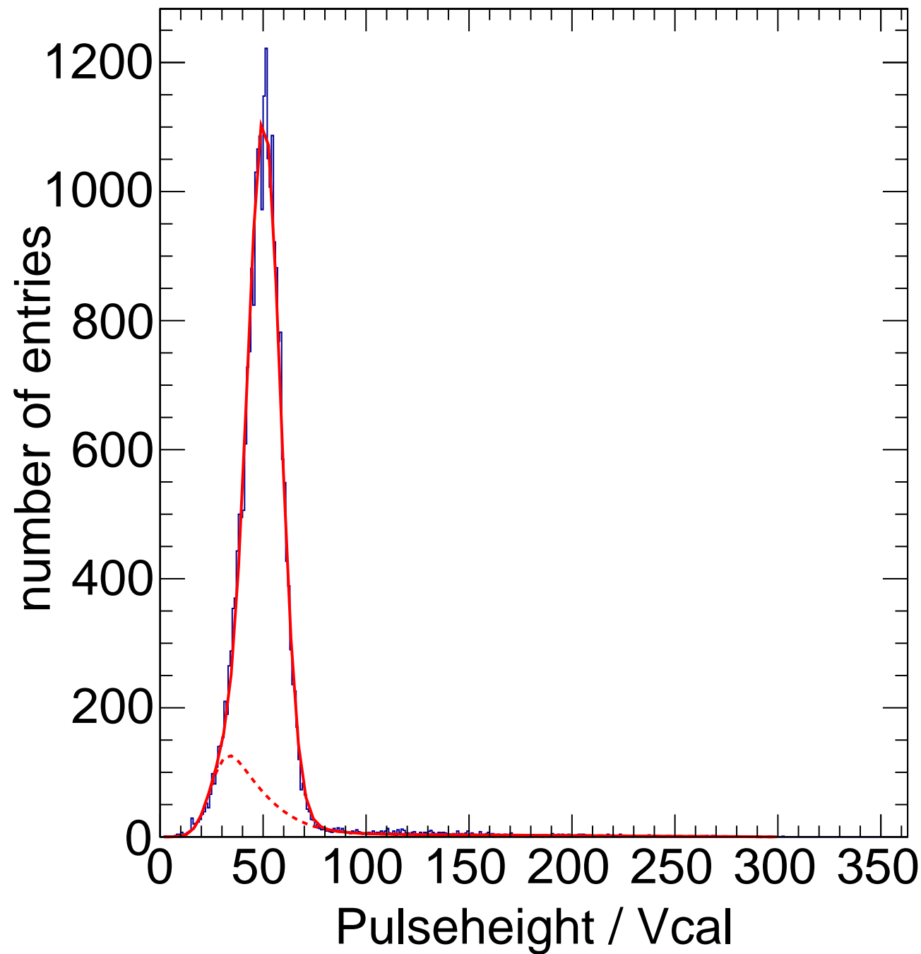
X-ray Calibration - Target Zn Method Spectrum Chip C12
