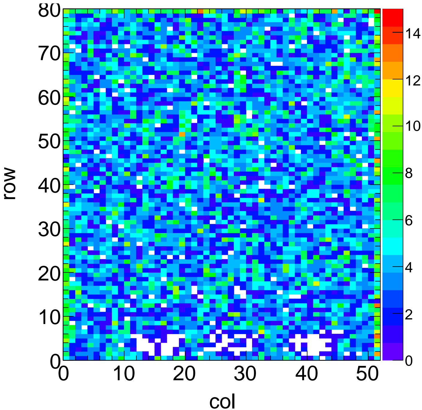
X-ray Hit Map - Target Sn Method Spectrum Chip C7
