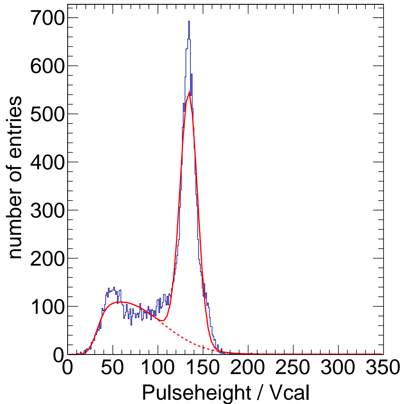
X-ray Calibration - Target Ag Method Spectrum Chip C6
