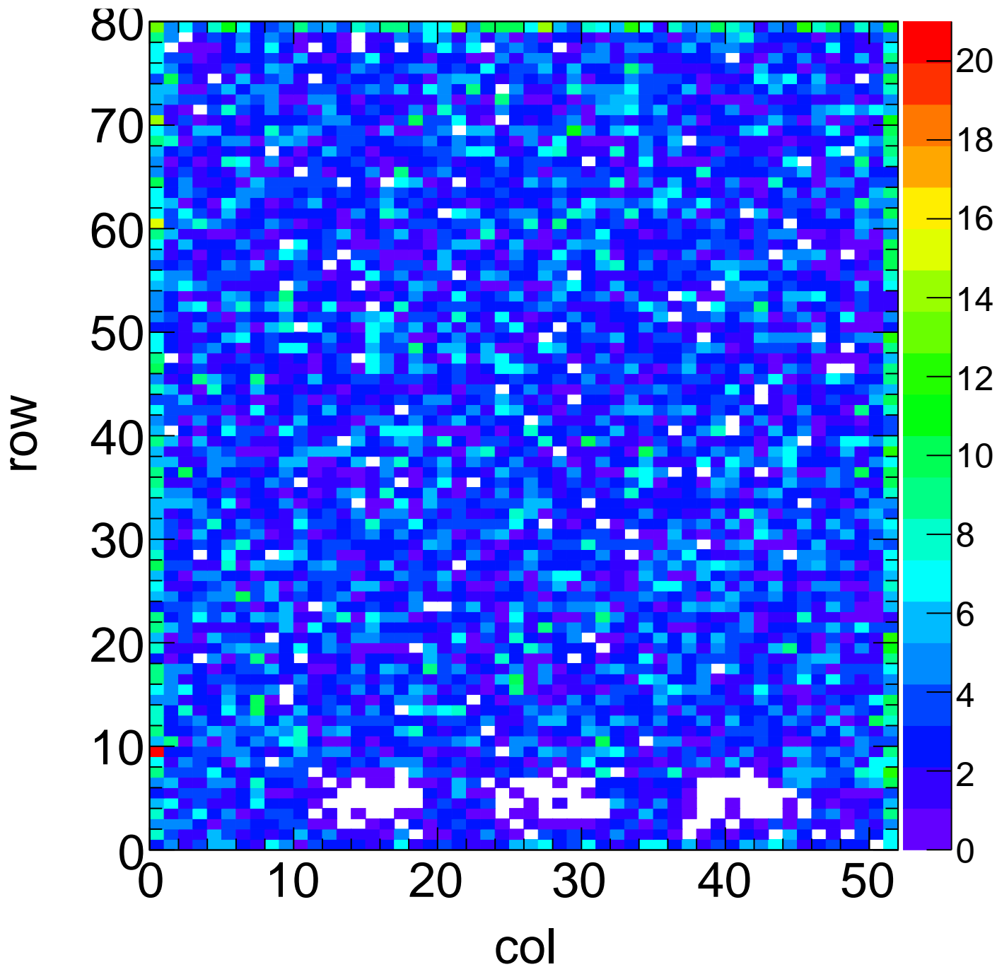
X-ray Hit Map - Target Sn Method Spectrum Chip C12
