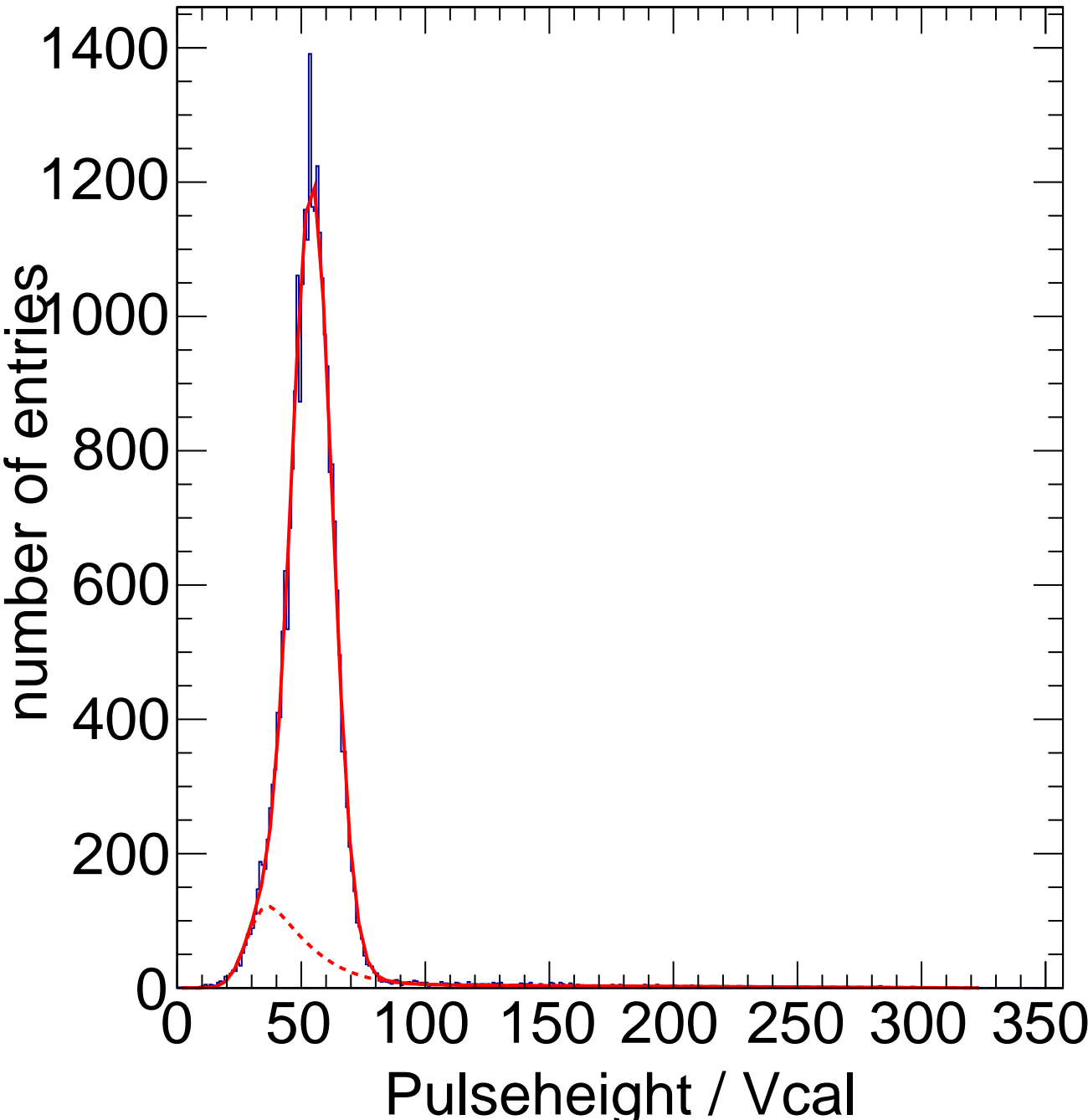
X-ray Calibration - Target Zn Method Spectrum Chip C3
