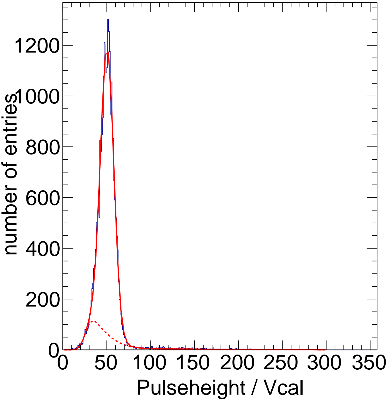
X-ray Calibration - Target Zn Method Spectrum Chip C9
