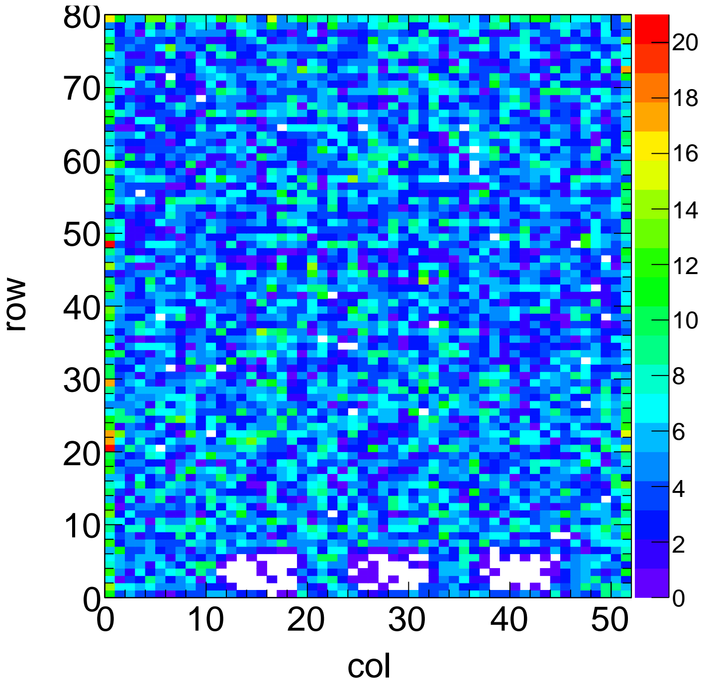
X-ray Hit Map - Target Ag Method Spectrum Chip C1
