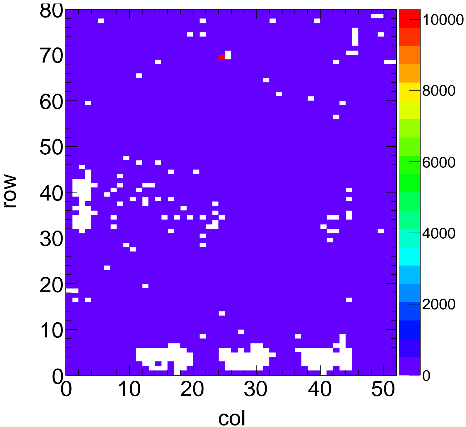
X-ray Hit Map - Target Zn Method Spectrum Chip C0
