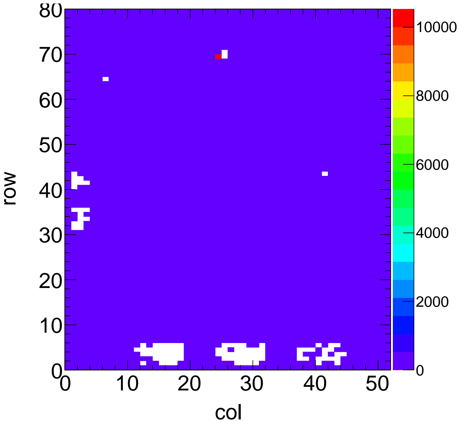
X-ray Hit Map - Target Mo Method Spectrum Chip C0
