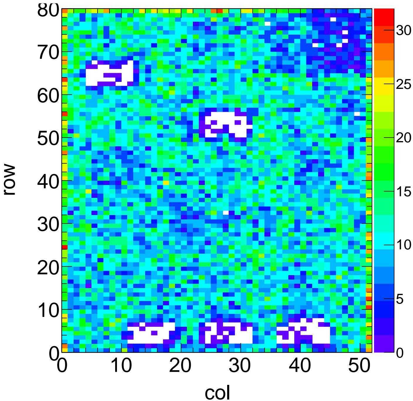
X-ray Hit Map - Target Mo Method Spectrum Chip C9
