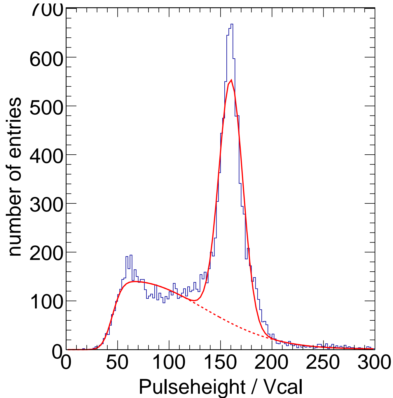
X-ray Calibration - Target Sn Method Spectrum Chip C15
