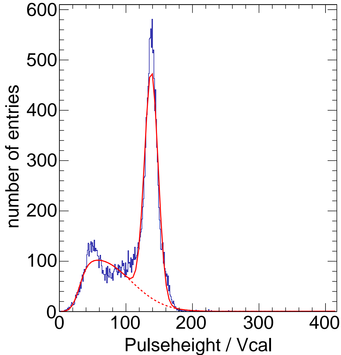
X-ray Calibration - Target Ag Method Spectrum Chip C4
